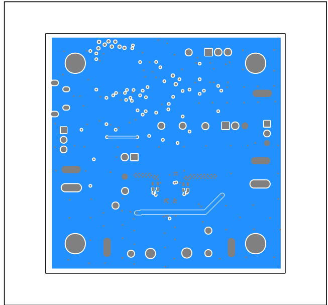
MAX77950 EV Kit PCB Layout—Bottom Layer
