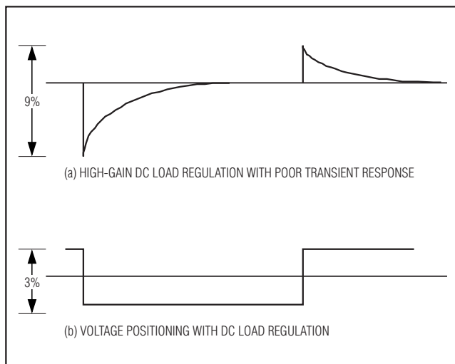
Figure 4. Transient-Response Comparison
