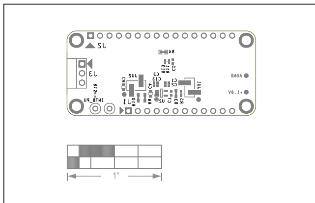
MAX86916 EV System—Bottom Silkscreen
