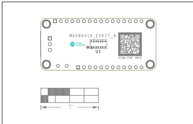
MAX86916 EV System—Top Silkscreen
