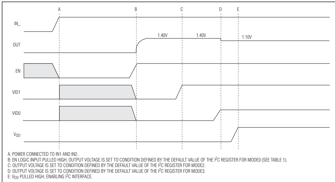
Figure 2. Power-Up Sequence
