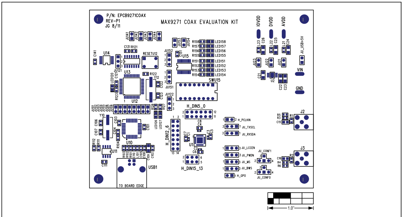
Figure 11. MAX9271 Coax EV Kit Component Placement Guide—Component Side
