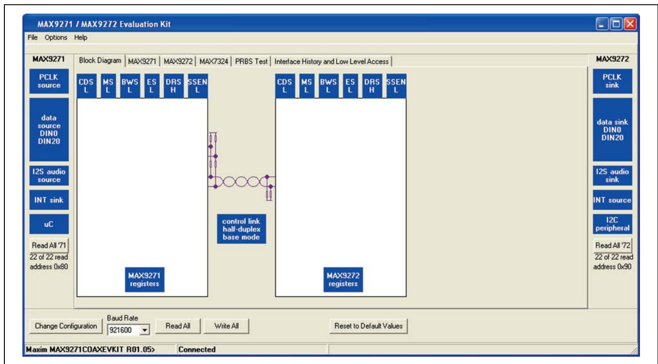
Figure 1. MAX9271/MAX9272 EV Kit Software Main Window (Block Diagram Tab)
