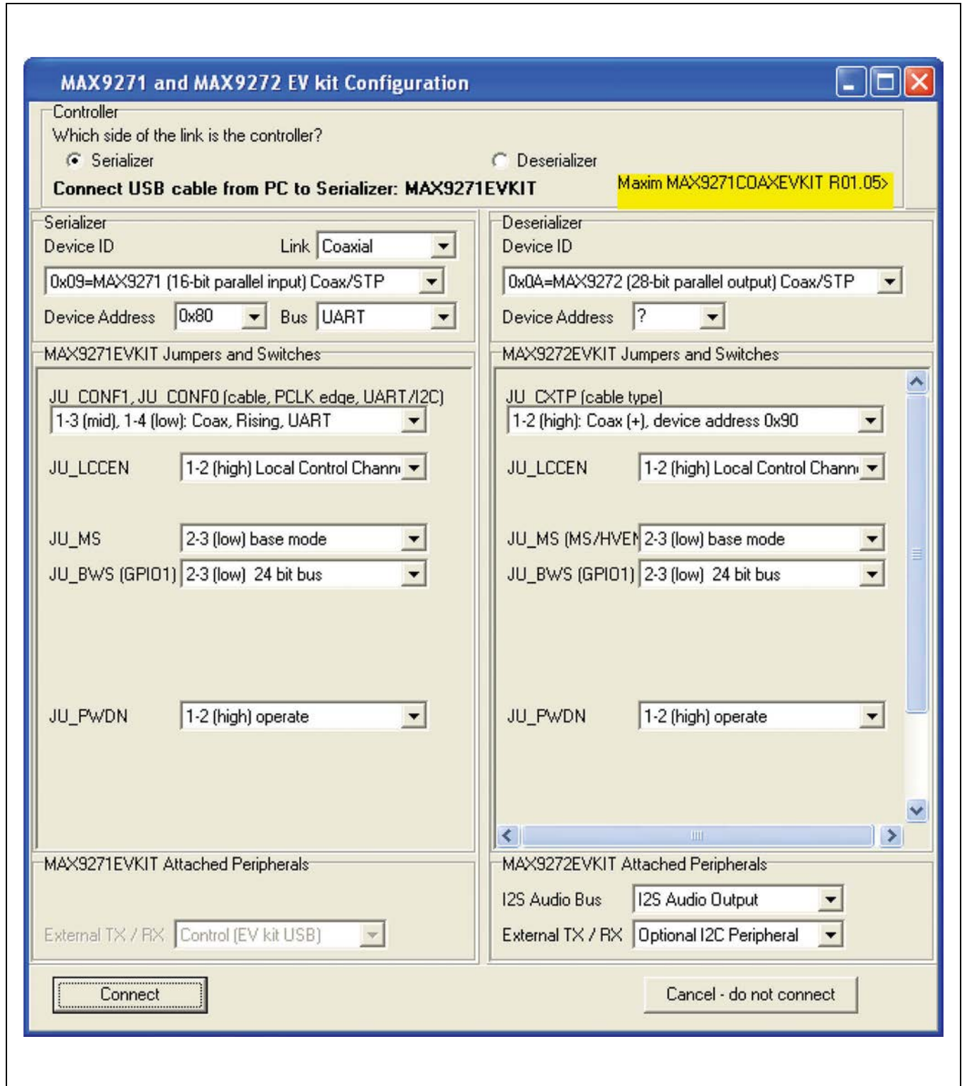
Figure 7. MAX9271/MAX9272 EV Kit Software Connect Window
