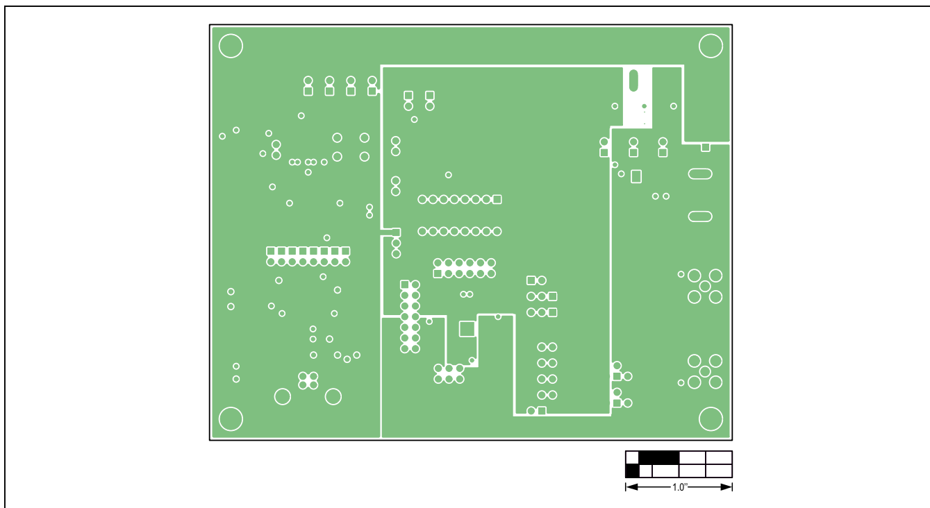
Figure 14. MAX9271 Coax EV Kit PCB Layout—Power Layer 3
