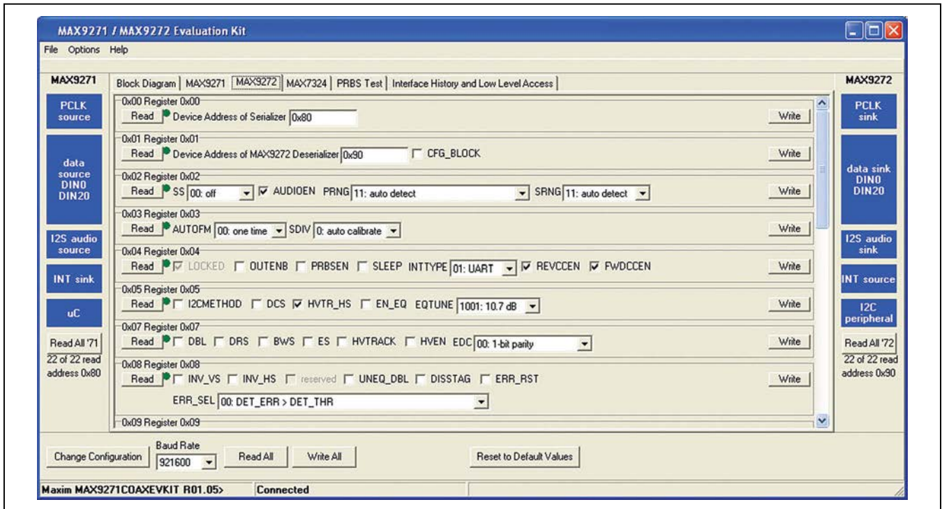
Figure 3. MAX9271/MAX9272 EV Kit Software Main Window (MAX9272 Tab)
