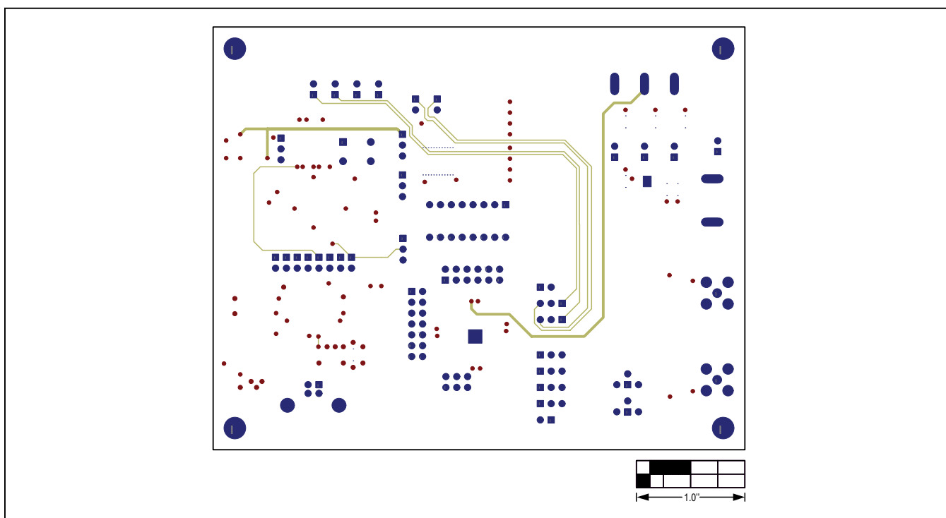
Figure 15. MAX9271 Coax EV Kit PCB Layout—Solder Side
