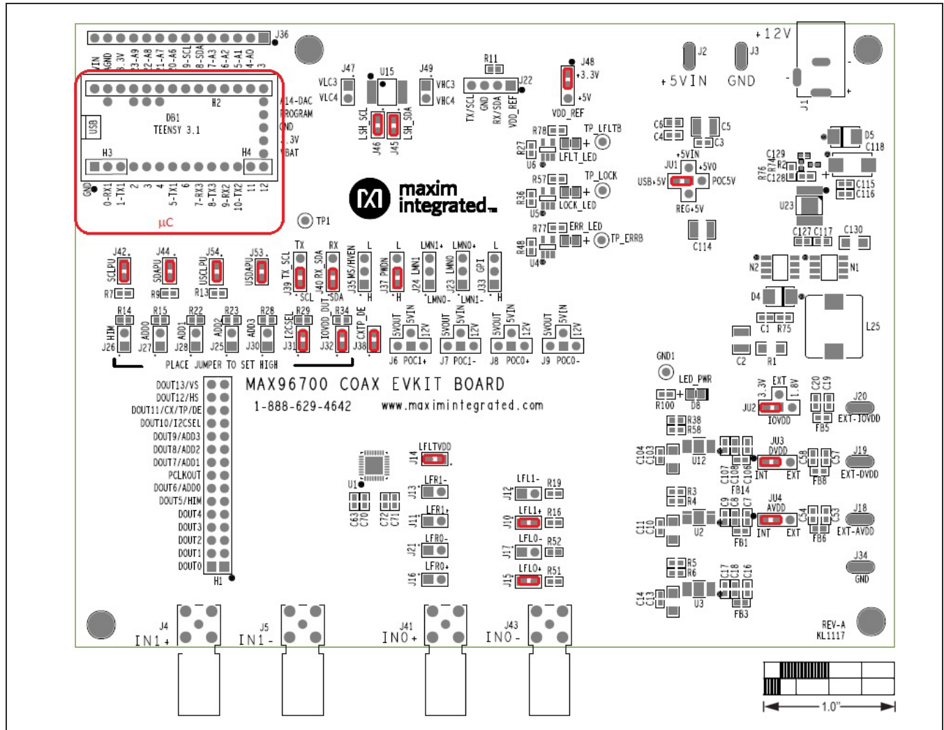
Figure 16. MAX96700 Coax EV Kit Jumper Settings for Coax Link and I 2 C Communication
