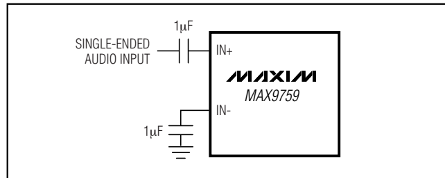
Figure 6. Single-Ended Input
