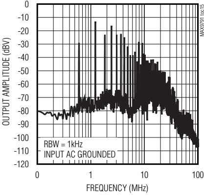
WIDEBAND OUTPUT SPECTRUM (SPEAKER MODE)
