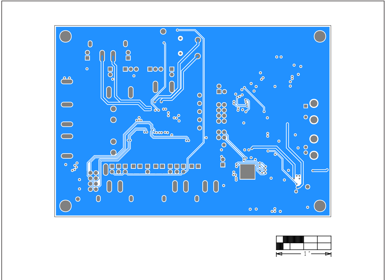
MAX98091 TQFN EV Kit PCB Layout—Bottom Layer
