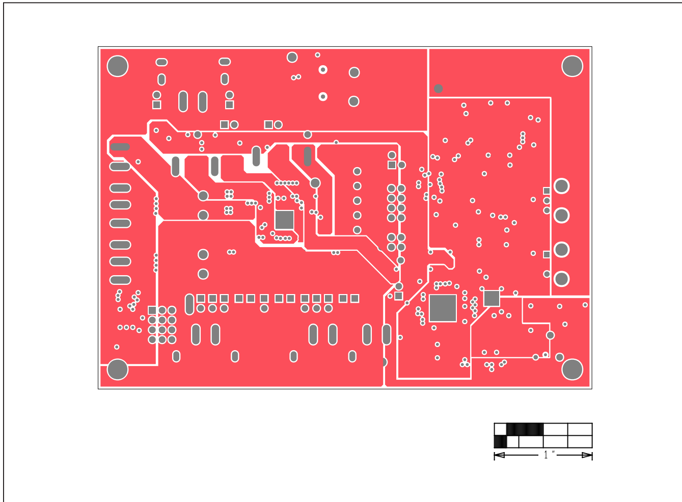
MAX98091 TQFN EV Kit PCB Layout—Internal Layer 4 VDD
