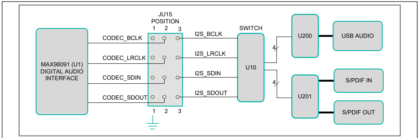
Figure 12. I 2 S Routing
