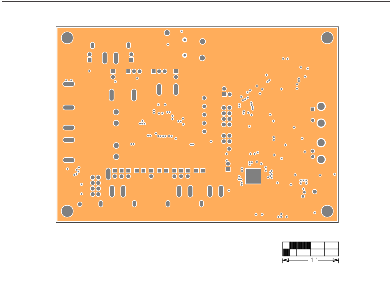
MAX98091 TQFN EV Kit PCB Layout—Internal Layer 5 GND1
