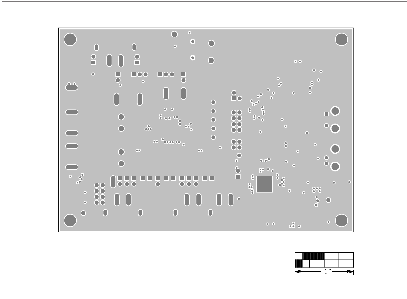
MAX98091 TQFN EV Kit PCB Layout—Internal Layer 2 GND
