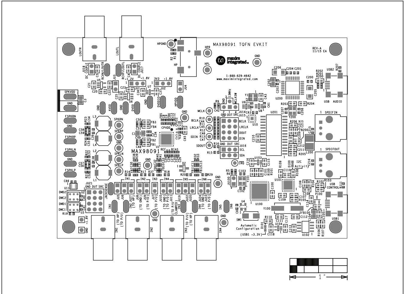
MAX98091 TQFN EV Kit Component Placement Guide—Top Silkscreen
