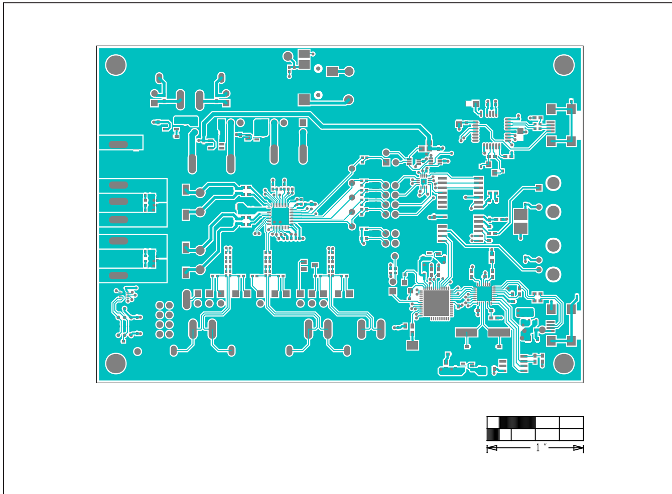
MAX98091 TQFN EV Kit PCB Layout—Top Layer
