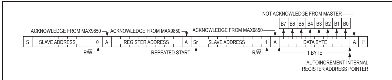
Figure 10. Reading One Byte of Data from MAX9850
