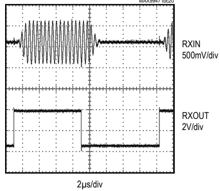
RECEIVER PROPAGATION DELAY AT 115.2kbps
