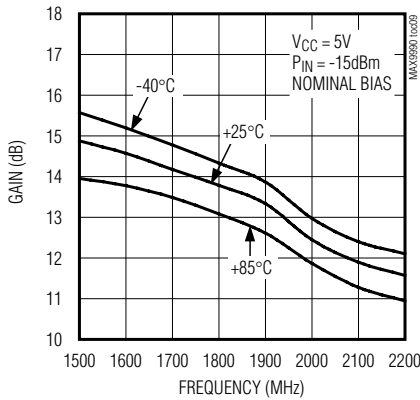
SMALL-SIGNAL GAIN vs. FREQUENCY OUTLO
