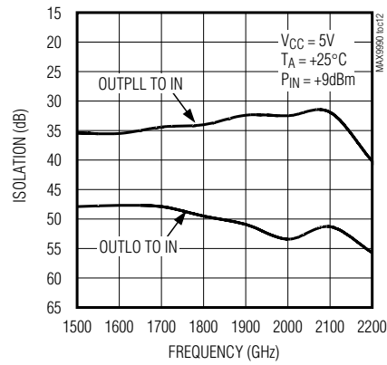
OUT-TO-IN ISOLATION vs. FREQUENCY
