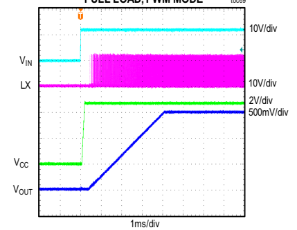
MAXM15067 STARTUP THROUGH V_{IN}
