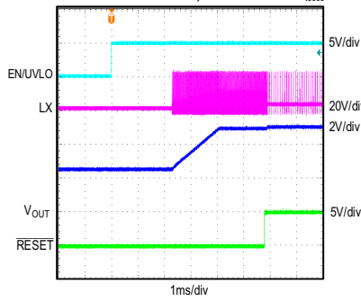
MAXM15066 STARTUP THROUGH ENABLE (2.5V PREBIAS)
