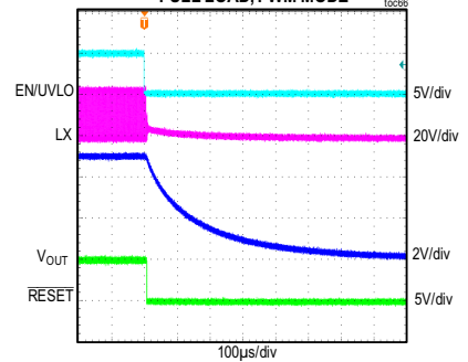
MAXM15066 SHUTDOWN THROUGH ENABLE
