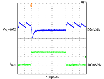
MAXM15463 LOAD TRANSIENT RESPONSE V_{IN} = 24V , FIXED V_{OUT} = 3.3V , PFM MODE (LOAD CURRENT STEPPED FROM 5mA TO 150mA)
