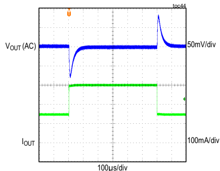
MAXM15462 LOAD TRANSIENT RESPONSE V_{IN} = 24V , ADJUSTABLE V_{OUT} = 5V , PWM MODE (LOAD CURRENT STEPPED FROM 150mA TO 300mA)
