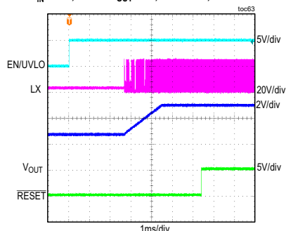
MAXM15464 STARTUP THROUGH ENABLE (2.5V PREBIAS) V_{IN} = 24V , FIXED V_{OUT} = 5V , NO LOAD, PWM MODE
