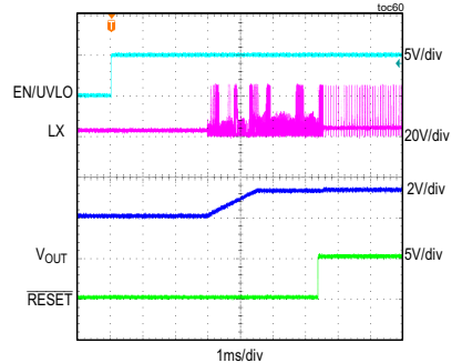
MAXM15463 STARTUP THROUGH ENABLE (2V PREBIAS) V_{IN} = 24V , FIXED V_{OUT} = 3.3V , NO LOAD, PFM MODE
