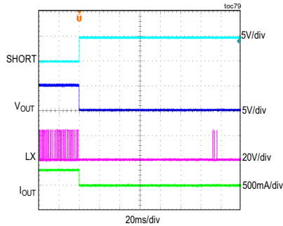
MAXM15464 OUTPUT SHORT IN STEADY STATE V_{IN} = 24V , FIXED V_{OUT} = 5V , FULL LOAD, PWM MODE
