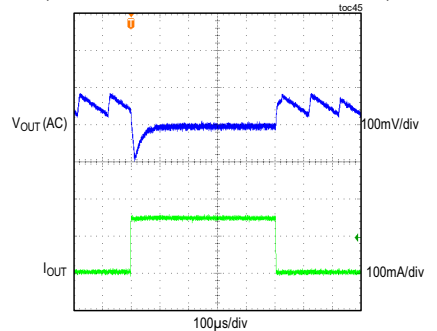
MAXM15463 LOAD TRANSIENT RESPONSE V_{IN} = 24V , FIXED V_{OUT} = 3.3V , PFM MODE (LOAD CURRENT STEPPED FROM 5mA TO 150mA)
