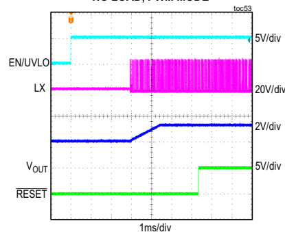
MAXM15462 STARTUP THROUGH ENABLE 2V PREBIAS, V_{IN} = 24V , ADJUSTABLE V_{OUT} = 3.3V , NO LOAD, PWM MODE
