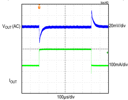
MAXM15462 LOAD TRANSIENT RESPONSE V_{IN} = 12V , ADJUSTABLE V_{OUT} = 1.5V , PWM MODE (LOAD CURRENT STEPPED FROM 150mA TO 300mA)
