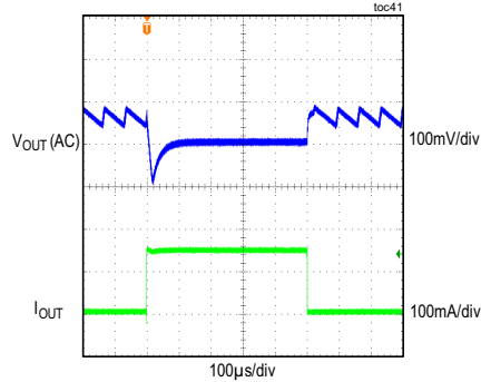
MAXM15462 LOAD TRANSIENT RESPONSE V_{IN} = 24V , ADJUSTABLE V_{OUT} = 3.3V , PFM MODE (LOAD CURRENT STEPPED FROM 5mA TO 150mA)
