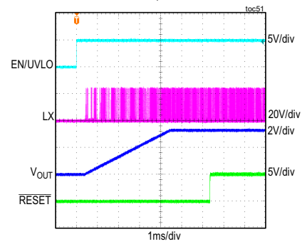
MAXM15462 STARTUP THROUGH ENABLE V_{IN} = 24V , ADJUSTABLE V_{OUT} = 3.3V , FULL LOAD, PWM MODE
