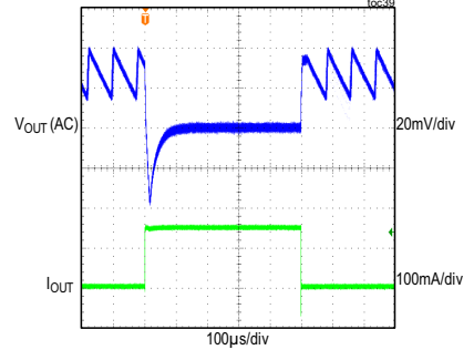
MAXM15462 LOAD TRANSIENT RESPONSE V_{IN} = 12V , ADJUSTABLE V_{OUT} = 1.5V , PFM MODE (LOAD CURRENT STEPPED FROM 5mA TO 150mA)
