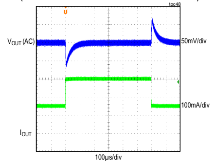
MAXM15464 LOAD TRANSIENT RESPONSE V_{IN} = 24V , FIXED V_{OUT} = 5V , PWM MODE (LOAD CURRENT STEPPED FROM 150mA TO 300mA)
