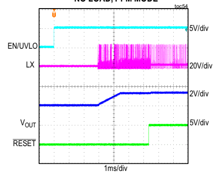
MAXM15462 STARTUP THROUGH ENABLE (2V PREBIAS) V_{IN} = 24V , ADJUSTABLE V_{OUT} = 3.3V , NO LOAD, PFM MODE
