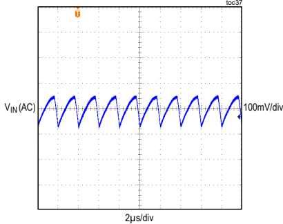
MAXM15463 INPUT VOLTAGE RIPPLE V_{IN} = 24V , FIXED V_{OUT} = 3.3V , FULL LOAD, PWM MODE
