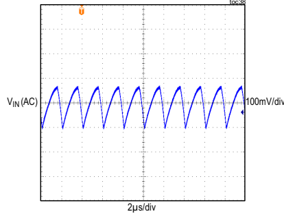
MAXM15464 INPUT VOLTAGE RIPPLE V_{IN} = 24V , FIXED V_{OUT} = 5V , FULL LOAD, PWM MODE
