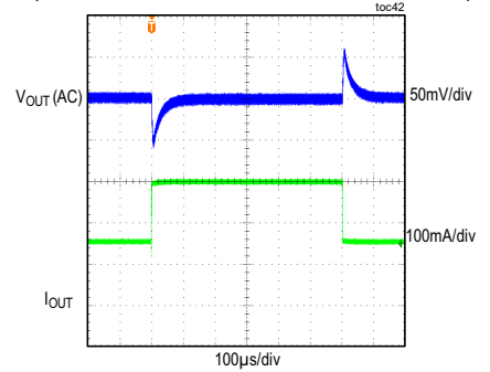
MAXM15462 LOAD TRANSIENT RESPONSE V_{IN} = 24V , ADJUSTABLE V_{OUT} = 3.3V , PWM MODE (LOAD CURRENT STEPPED FROM 150mA TO 300mA)
