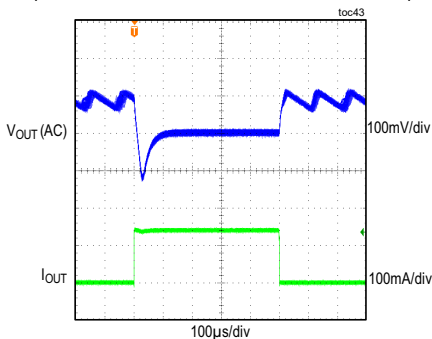
MAXM15462 LOAD TRANSIENT RESPONSE V_{IN} = 24V , ADJUSTABLE V_{OUT} = 5V , PFM MODE (LOAD CURRENT STEPPED FROM 5mA TO 150mA)
