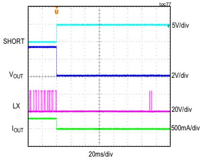
MAXM15463 OUTPUT SHORT IN STEADY STATE V_{IN} = 24V , FIXED V_{OUT} = 3.3V , FULL LOAD, PWM MODE
