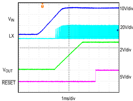
STARTUP THROUGH INPUT SUPPLY V_{IN} = 24V, V_{OUT} = 5V, I_{OUT} = 1.7A, MODE = SGND toc37
