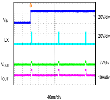
OUTPUT SHORT DURING STARTUP VIN = 24V, VOUT = 3.3V, IOUT = SHORT, MODE = SGND
