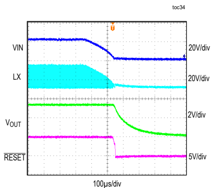
SHUTDOWN THROUGH INPUT SUPPLY V_{IN} = 24V, V_{OUT} = 3.3V, I_{OUT} = 1.7A, MODE = SGND
