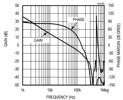
CLOSED-LOOP BODE PLOT VIN = 24V, VOUT = 3.3V, IOUT = 1.7A, MODE = SGND
