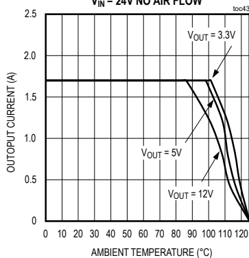
OUTPUT CURRENT vs. AMBIENT TEMPERATURE VIN = 24V NO AIR FLOW
