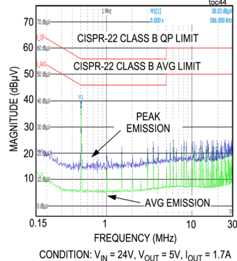
CONDUCTED EMISSION PLOT WITH FILTER: C4 = 2.2µF, L1 = 10µH, C14 = 2.2µF
