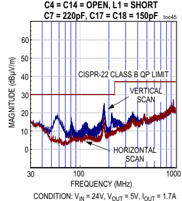
RADIATED EMISSION PLOT C4 = C14 = OPEN, L1 = SHORT C7 = 220pF, C17 = C18 = 150pF
