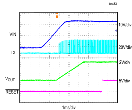
STARTUP THROUGH INPUT SUPPLY V_{IN} = 24V, V_{OUT} = 3.3V, I_{OUT} = 1.7A, MODE = SGND
