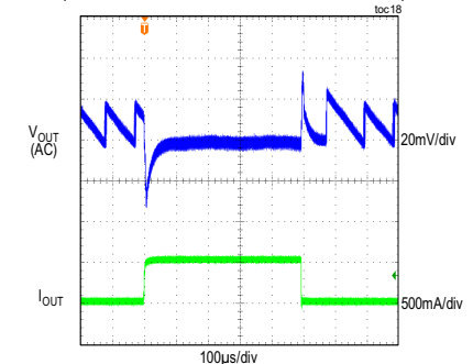
MAXM17623 LOAD TRANSIENT RESPONSE ( V_{IN} = 5V , V_{OUT} = 0.8V , PFM MODE) (LOAD CURRENT STEPPED FROM 0A TO 0.5A)
