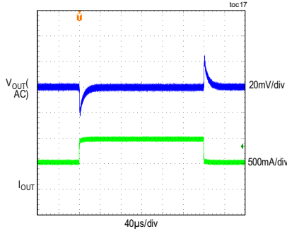
MAXM17623 LOAD TRANSIENT RESPONSE ( V_{IN} = 5V , V_{OUT} = 0.8V , PWM MODE) (LOAD CURRENT STEPPED FROM 0.5A TO 1A)
