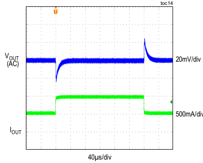
MAXM17623 LOAD TRANSIENT RESPONSE ( V_{IN} = 3.3V , V_{OUT} = 0.8V , PWM MODE) (LOAD CURRENT STEPPED FROM 0.5A TO 1A)
