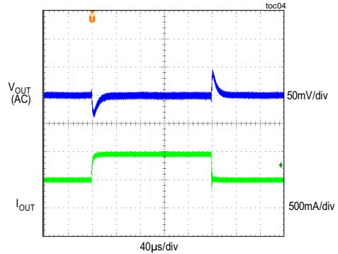
MAXM17623 LOAD TRANSIENT RESPONSE V_{IN} = 3.3V , V_{OUT} = 1.5V , MODE = PWM (LOAD CURRENT STEPPED FROM 0.5 TO 1A)
