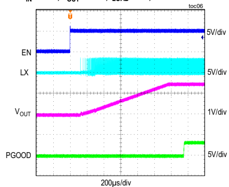
MAXM17623 STARTUP THROUGH ENABLE V_{IN} = 3.3V , V_{OUT} = 1.5V , I_{LOAD} = 1A , MODE = PWM
