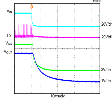
MAXM17632 SHUTDOWN THROUGH V_{IN} V_{OUT} = 2.5V , f_{SW} = 700kHz , 10mA LOAD, PFM MODE
