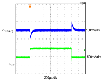
MAXM17631/MAXM17632 LOAD-TRANSIENT RESPONSE V_{OUT} = 5V , f_{SW} = 1250kHz , PWM MODE (LOAD CURRENT STEPPED FROM 0.5A TO 1A)
