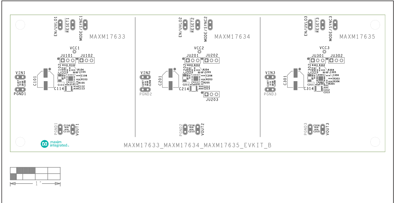
MAXM17633/MAXM17634/MAXM17635 EV Kits—Top Silkscreen
