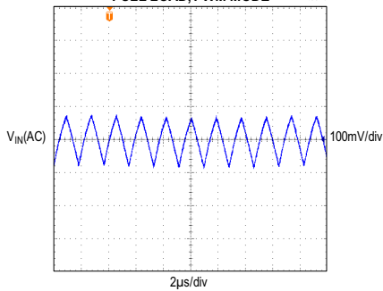
MAXM17906 INPUT VOLTAGE RIPPLE V_{IN} = 12V , ADJUSTABLE V_{OUT} = 5V , FULL LOAD, PWM MODE
