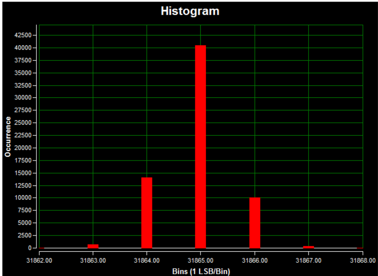
Figure 7. DC histogram using external power; a 5V input signal; a 20kps sample rate; 65,536 samples; a code spread of 7 LSBs with 98.5% of the codes falling within the three center LSBs; and a standard deviation of 0.651.
