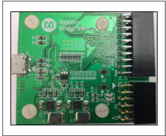
Figure 1. USB2GPIO# Board
