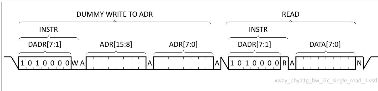
Figure 16 Timing Diagram for a Random Address Single Byte Read
