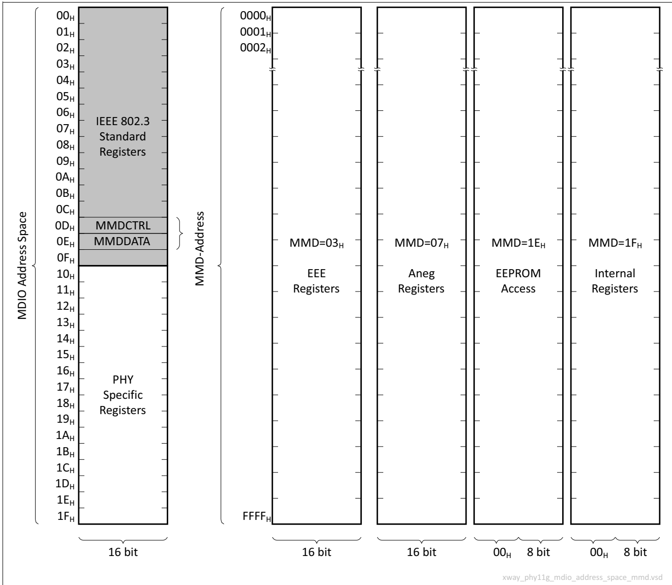
Figure 22 Layout of the MDIO Address Space
