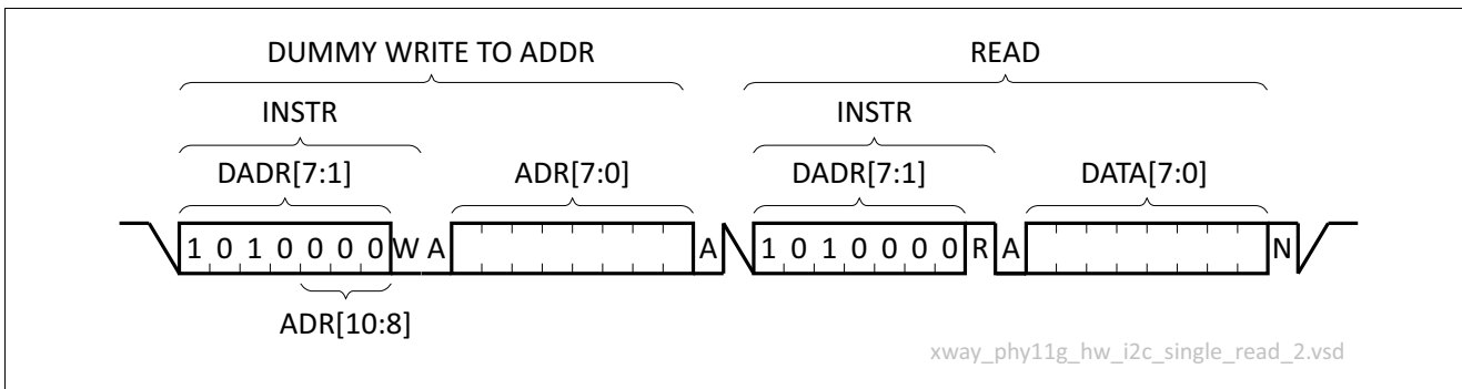
Figure 13 Timing Diagram for a Random Address Single Byte Read
