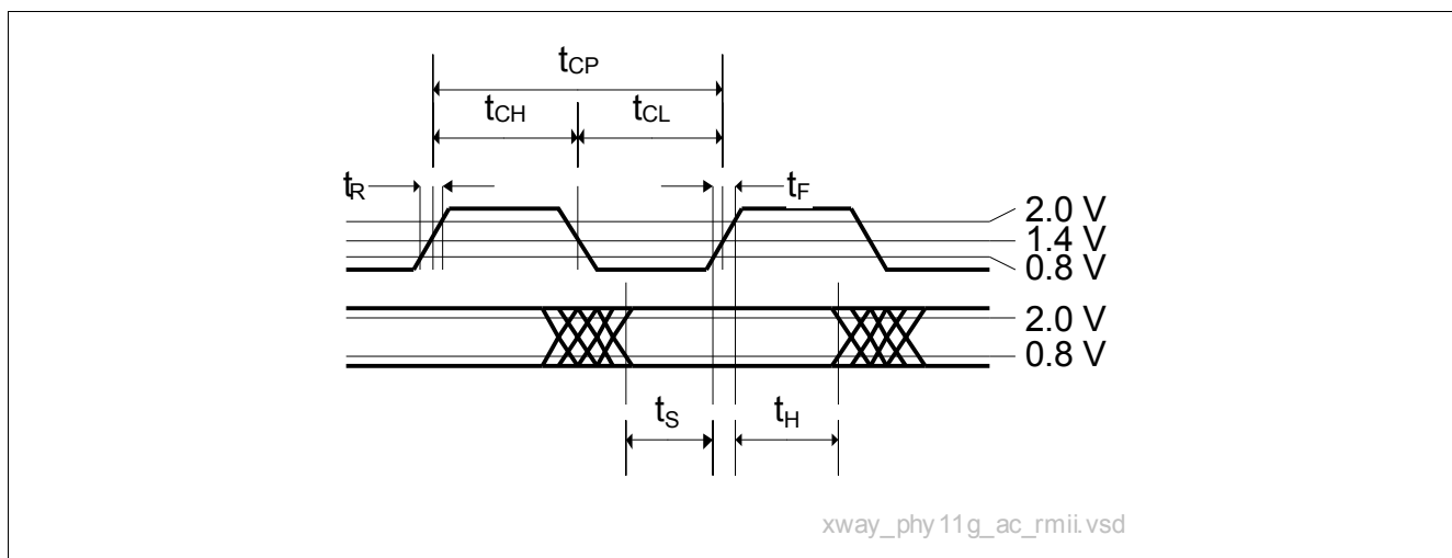
Figure 40 Transmit/Receive Timing Diagram of the RMI
