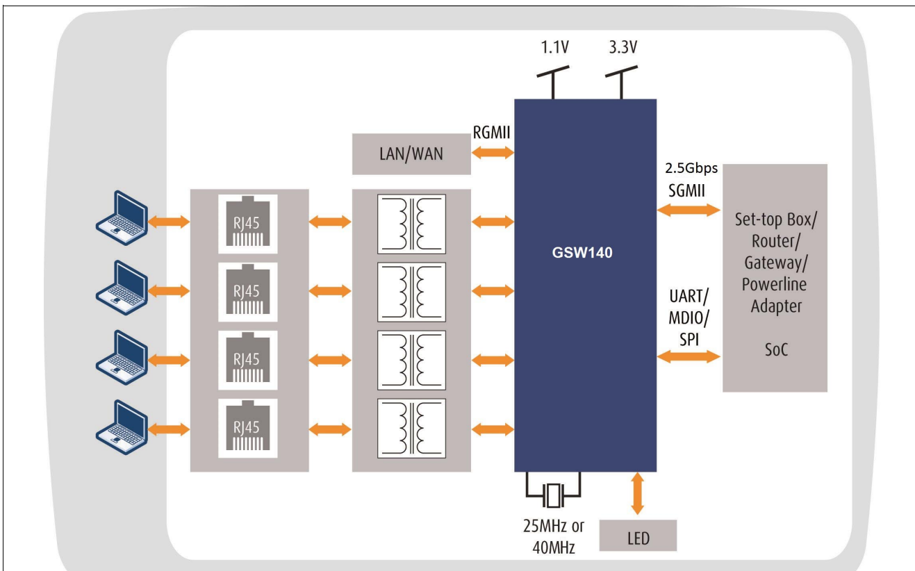
Figure 3 Home Gateway
