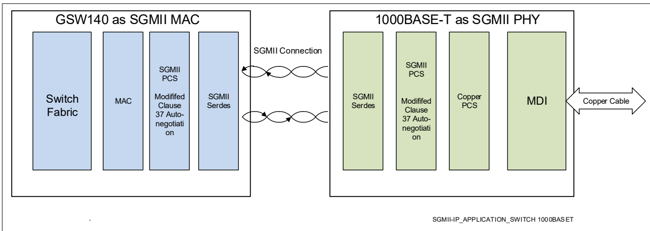
Figure 23 Interface to an External 1000BASE-T Copper Gigabit Ethernet PHY
