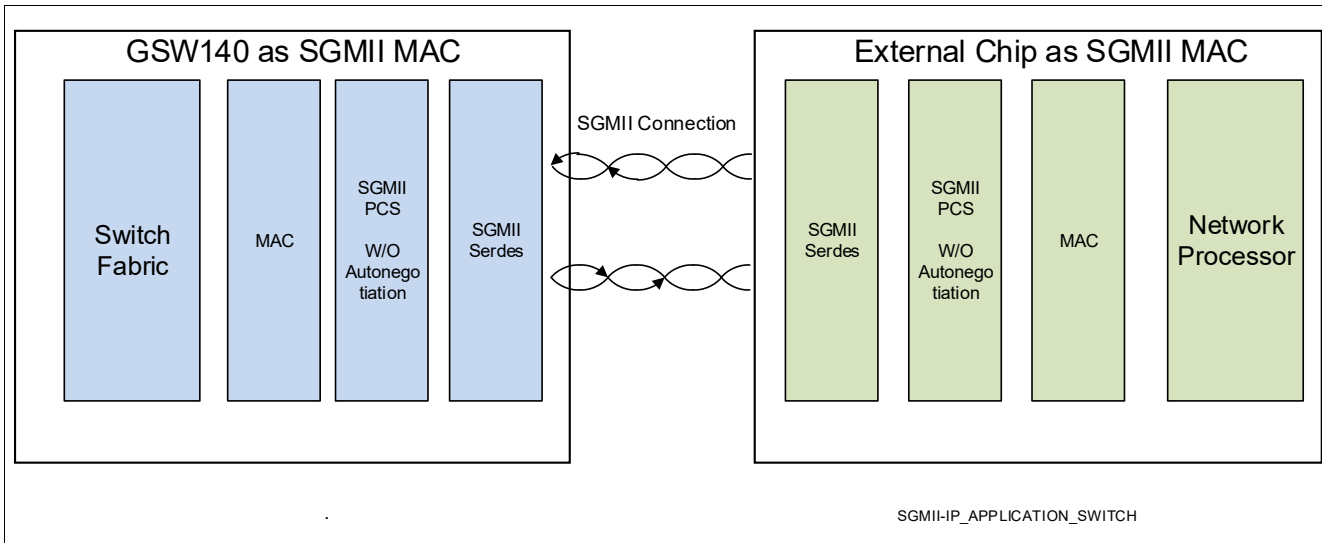
Figure 22 Interface to an External MAC
