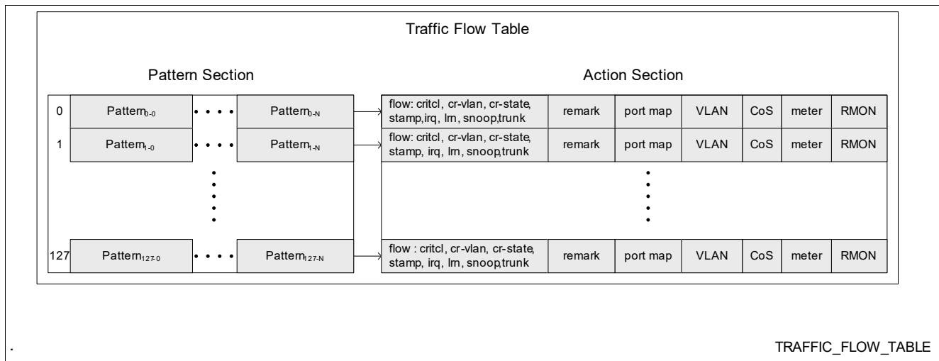
Figure 43 Traffic Flow Table
