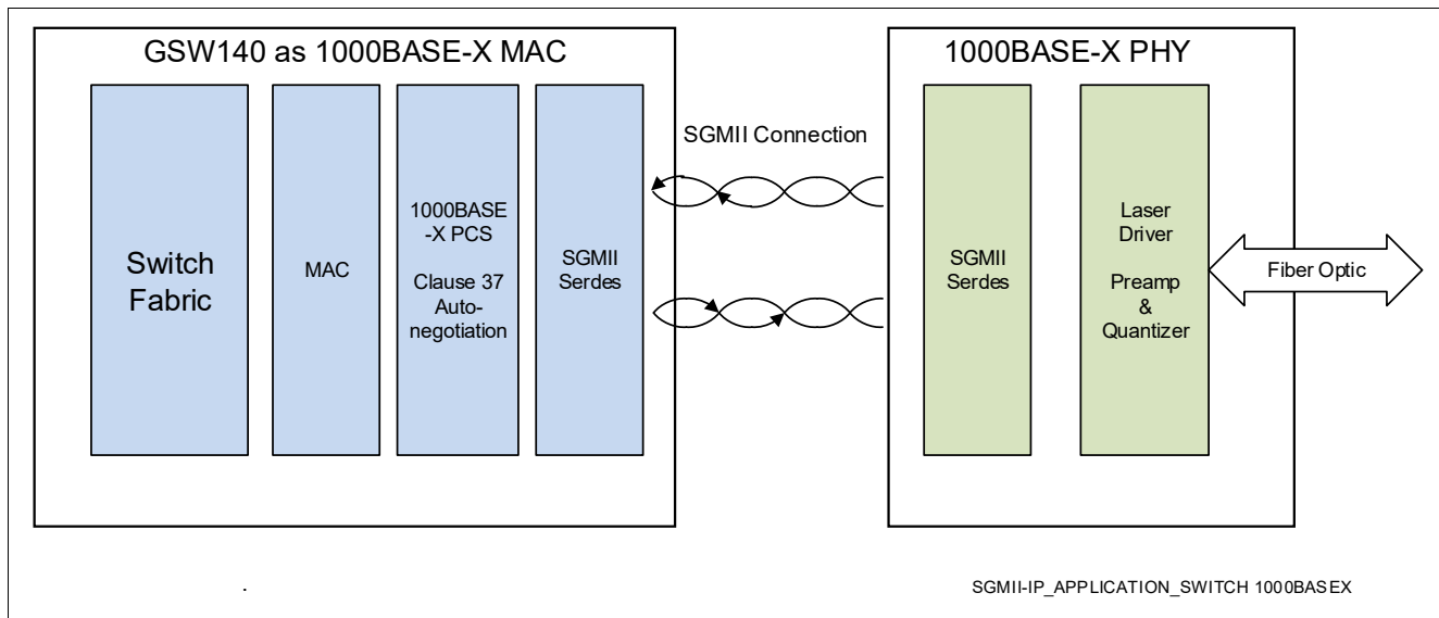
Figure 24 Interface to an External 1000BASE-X Ethernet PHY
