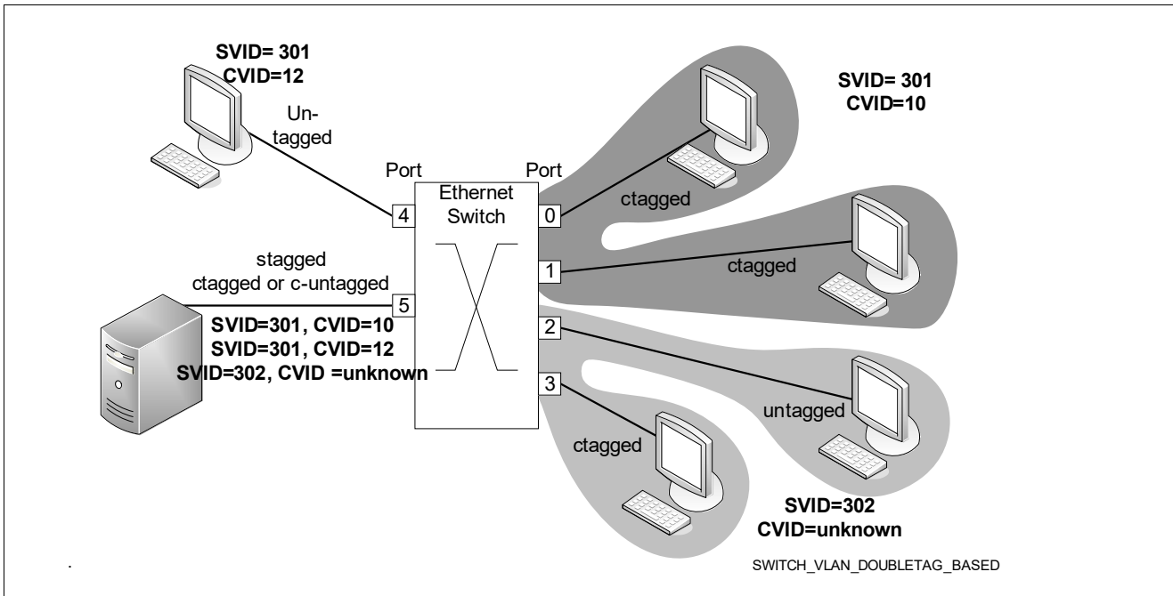
Figure 33 Double Tag and Port based VLAN Example
