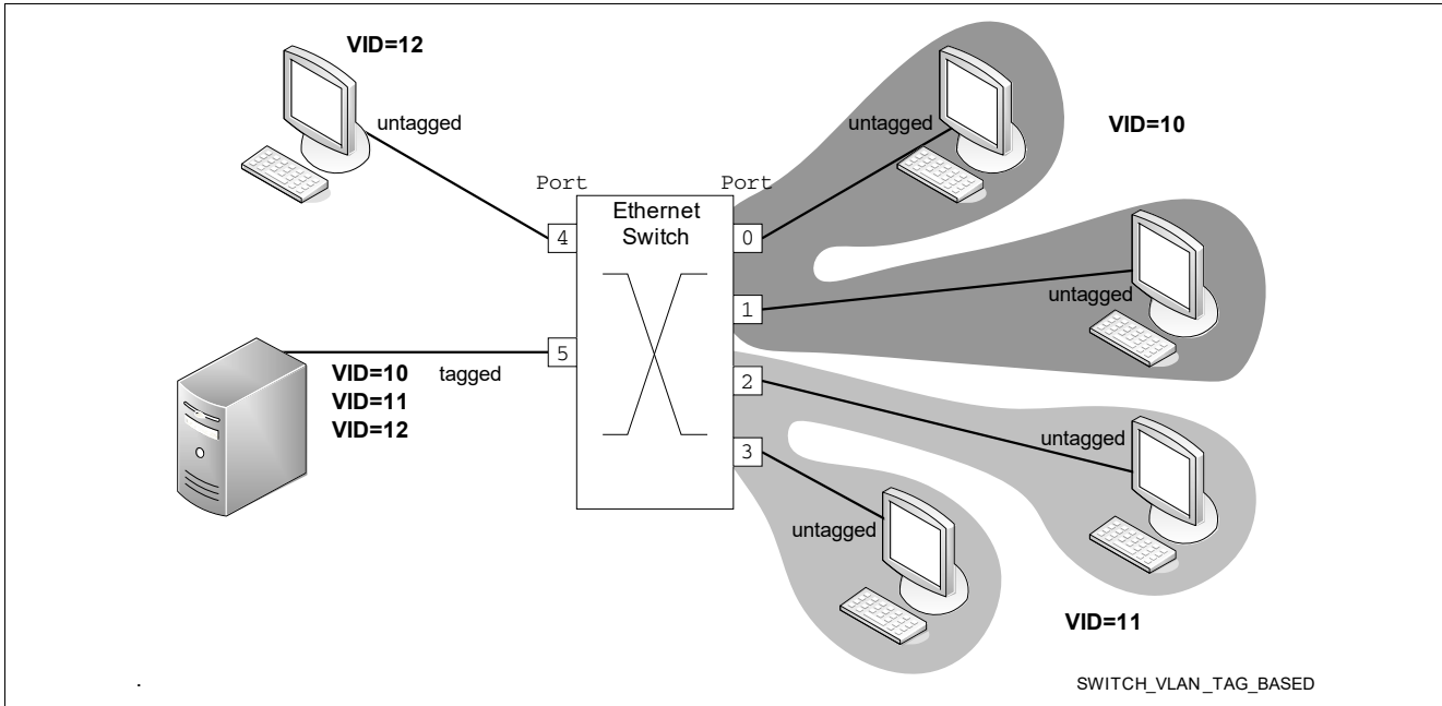
Figure 32 Tag-based VLAN Example
