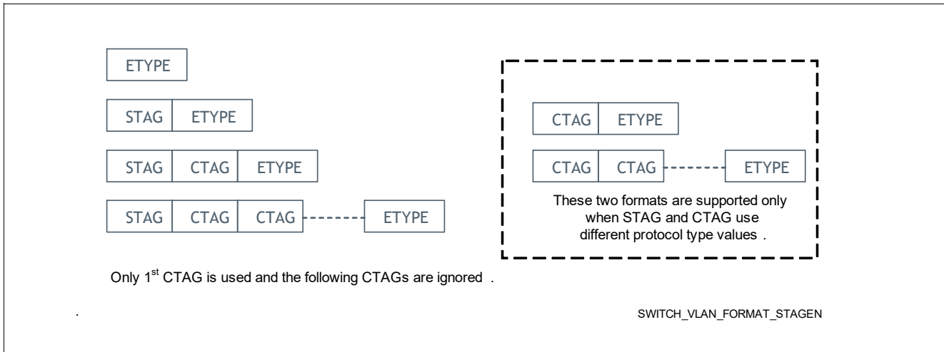
Figure 29 Supported Frame Formats when STAG is enabled
