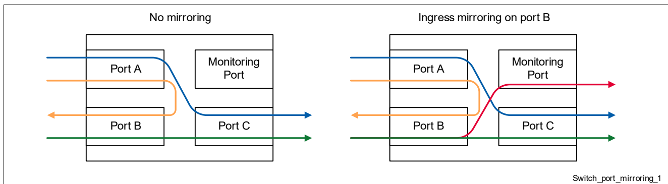
Figure 44 Port Mirroring Examples – Ingress Monitoring
