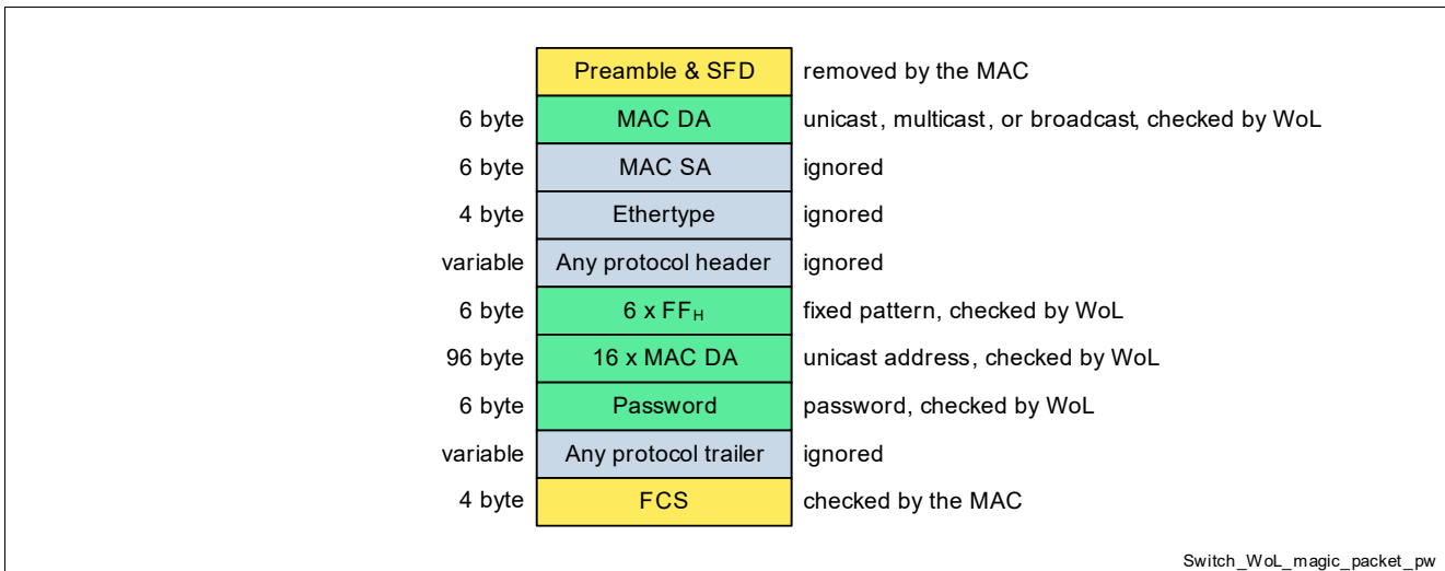
Figure 47 Magic Packet Data Structure – Password Protection
