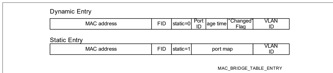
Figure 27 MAC Bridge Table Entry Formats
