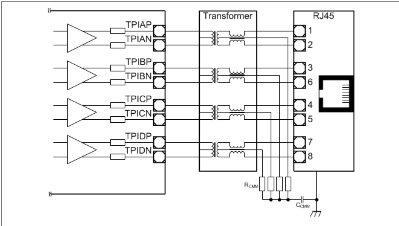
Figure 18 Twisted-Pair Interface of GPHY IP Including Transformer and RJ45 Plug
