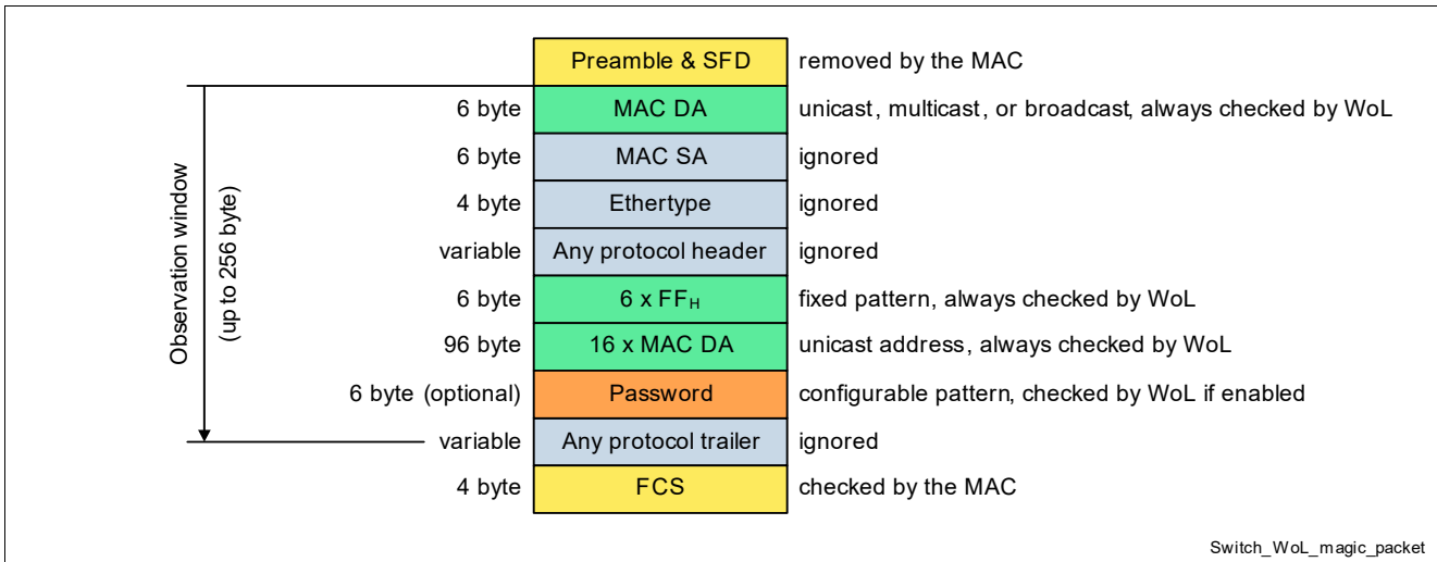
Figure 46 Typical Magic Packet Data Structure
