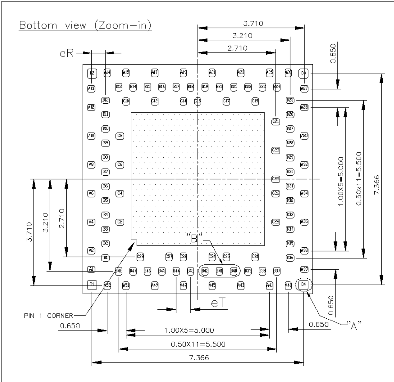
Figure 57 MRQFN 8 mm x 8 mm Package Outline
