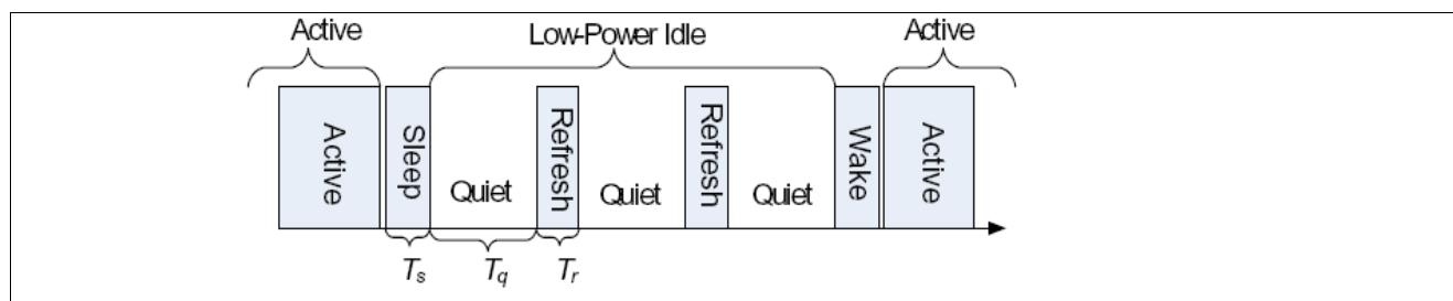
Figure 21 EEE Low-Power Idle Sequence
