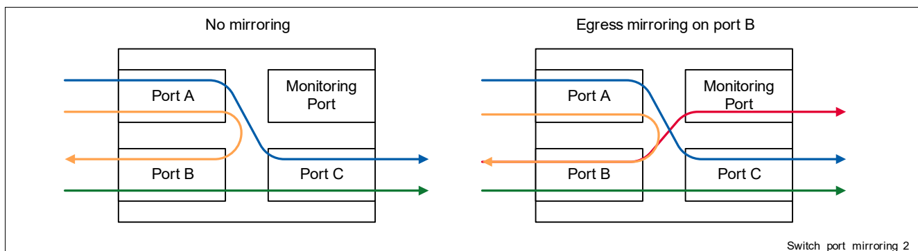
Figure 45 Port Mirroring Examples – Egress Monitoring
