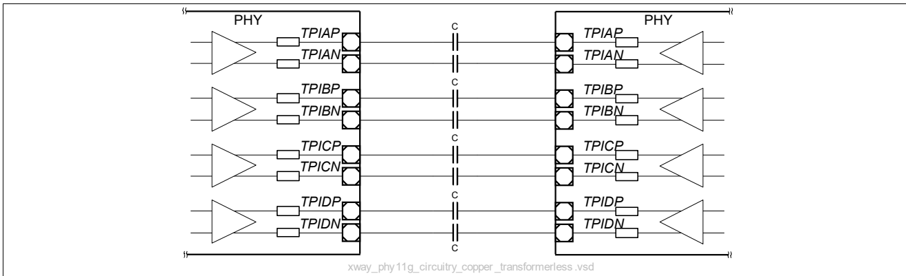
Figure 19 External Circuitry for the Transformerless Ethernet Application
