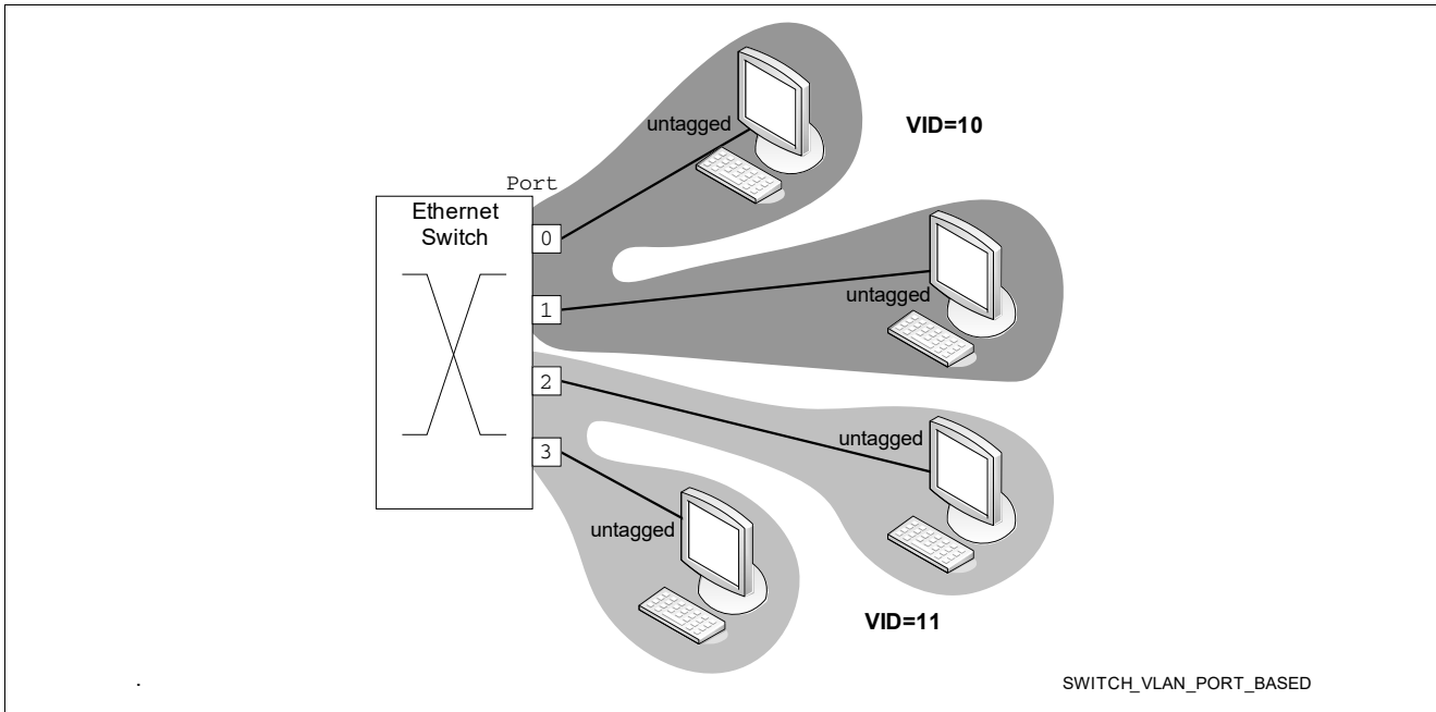
Figure 31 Port-based VLAN Example
