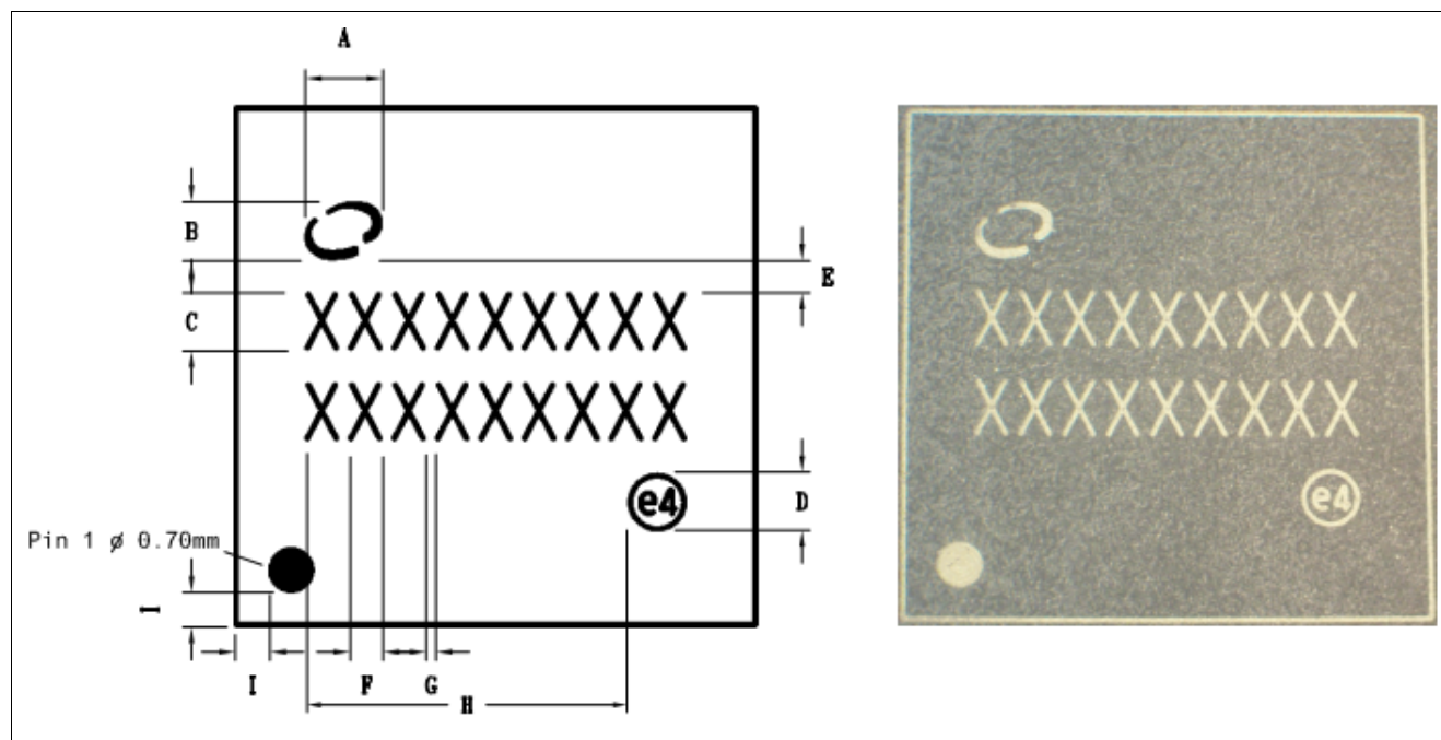
Figure 59 Chip Marking of GSW140
