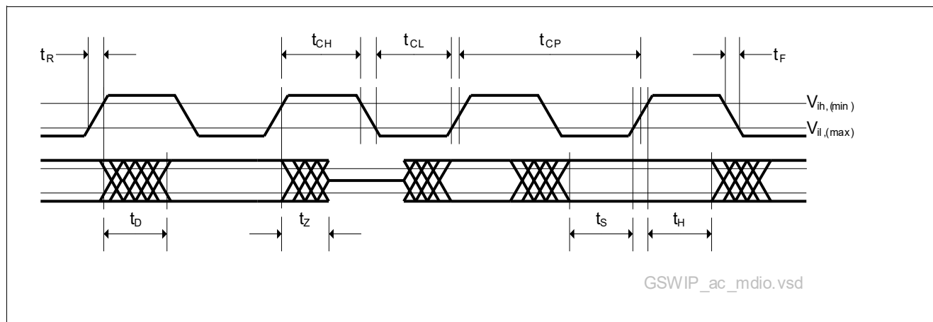
Figure 52 Timing Diagram for the SMDIO Interface
