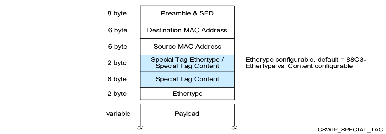
Figure 49 Special tag location in the frame
