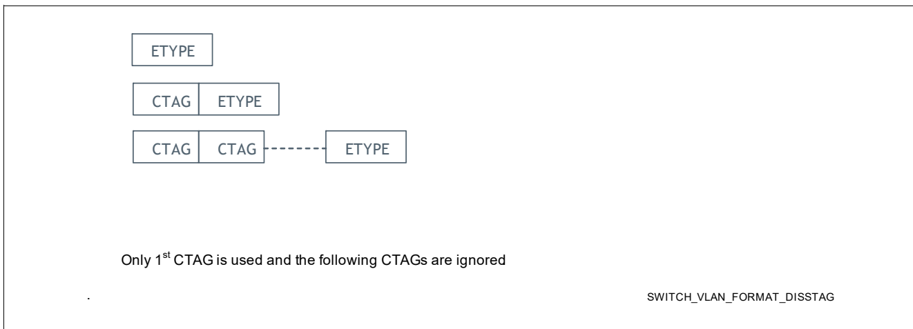
Figure 30 Supported Frame Formats when STAG is disabled
