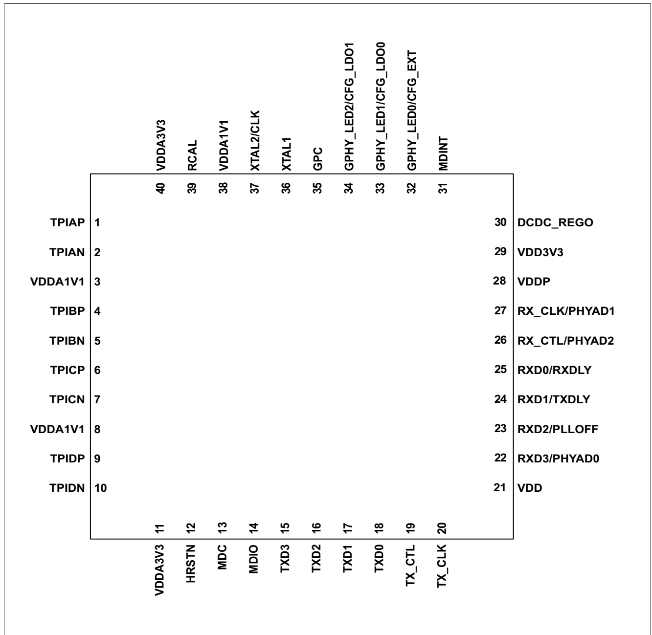
Figure 3 Pin Diagram for MxL86110
