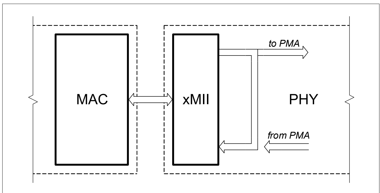
Figure 4 Near-End Loopback
