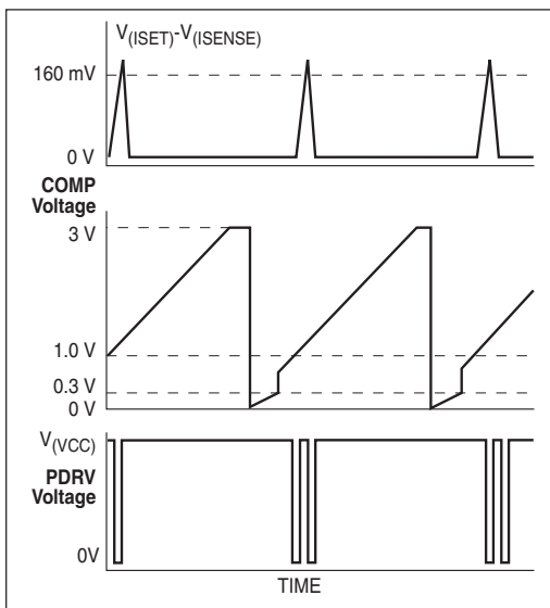
Figure 2. SP6121 Hiccup mode waveforms
