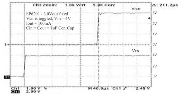
Fig. 23: Turn on time, I O =100mA, 4V IN
