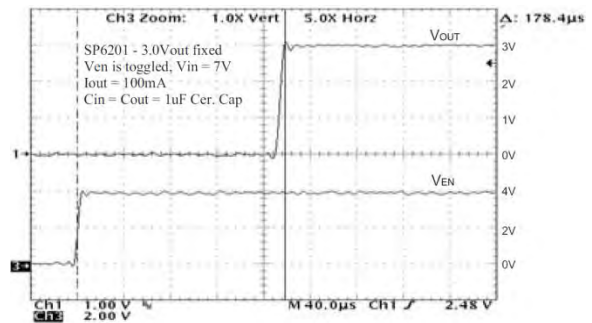
Fig. 25: Turn on time, I O =100mA, 7V IN
