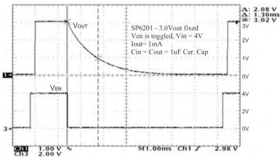
Fig. 26: Turn off time, I O =1mA, 4V IN
