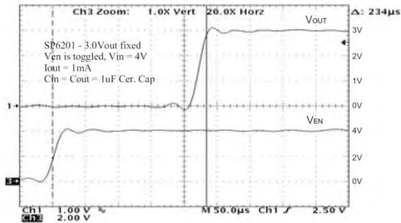
Fig. 22: Turn on time, I O =1mA, 4V IN
