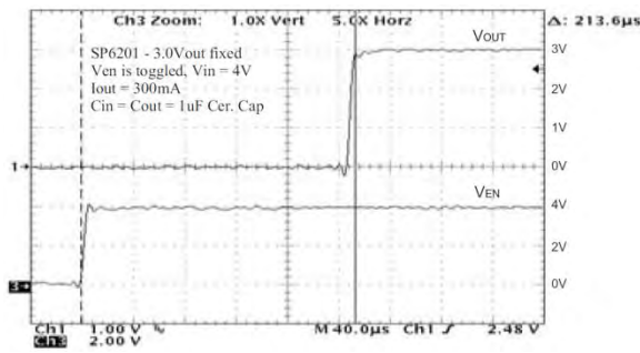
Fig. 24: Turn on time, I O =300mA, 4V IN
