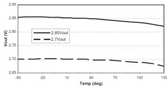
Fig. 14: V_{OUT} vs. Temp (adjustable)
