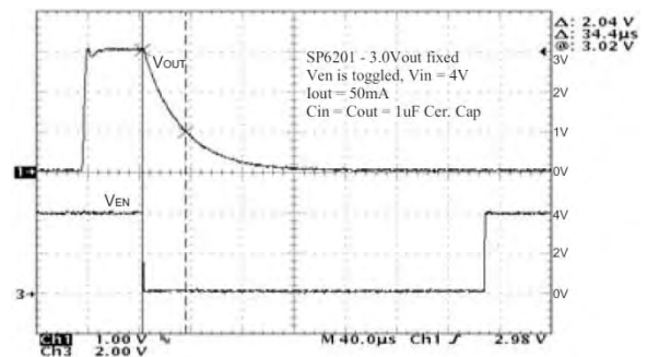
Fig. 27: Turn off time, I O =50mA, 4V IN
