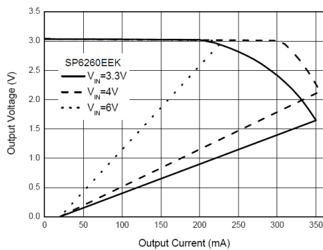
Fig. 8: Output Voltage vs. Output Current SP6260EEK (3.0V)
