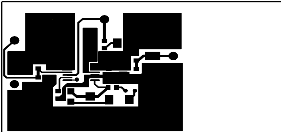
FIGURE 2: SP6648LEDEB PCB LAYOUT TOP SIDE
