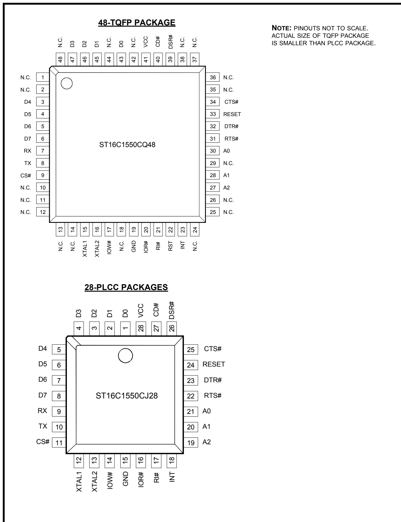
FIGURE 2. ST16C1550 PINOUTS
