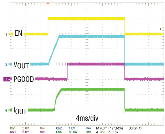
Figure 14. Enable Functionality, V_{IN} = 12V
