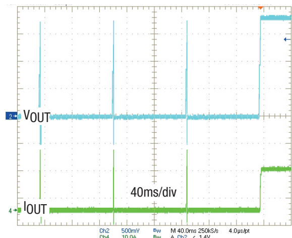
Figure 16. Short-Circuit Recovery, I_{OUT} = 15A
