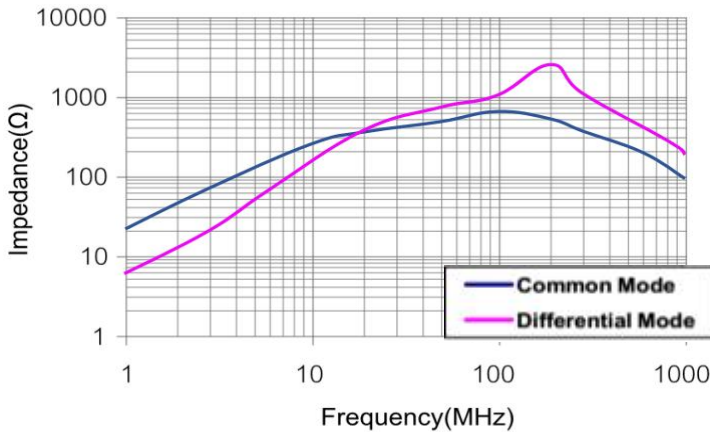
XRACM1211F-501
