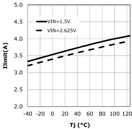
Fig. 8: Ilimit versus temperature
