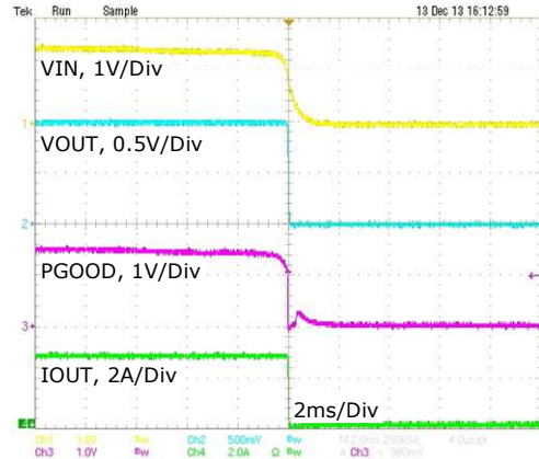
Fig. 11: Powerdown, IOU=3A, 1.5VIN, 1VOUT
