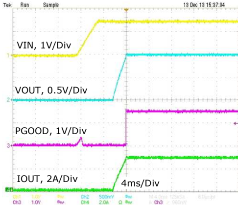
Fig. 10: Powerup, IOU=3A, 1.5VIN, 1VOUT
