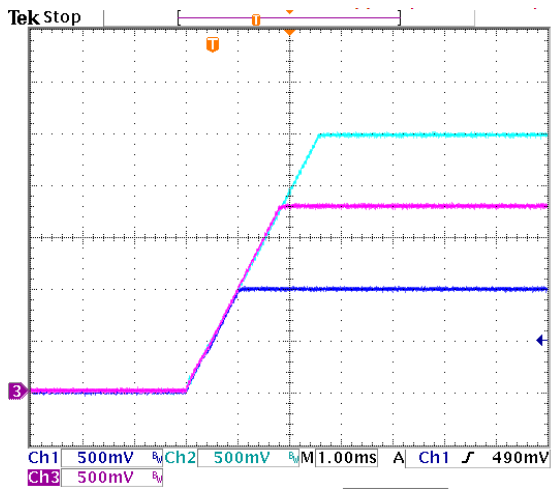
Fig. 12: CH1: 1.0V CH2:5V CH3: 1.8V Simultaneous Start-up Configuration
