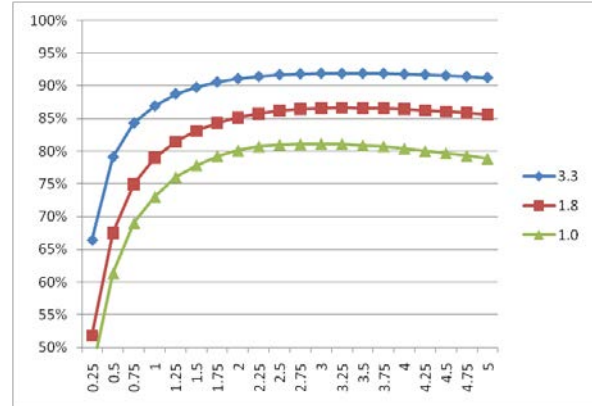
Fig. 5: 12Vin Efficiency: Single Channel 300kHz - Channels not in use are disabled FET: FDS8984; Inductor: 744310200 7x7x3mm
