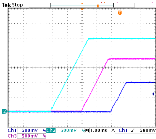
Fig. 14: CH1: 1.0V CH2:5V CH3: 1.8V Sequential Start-up Configuration
