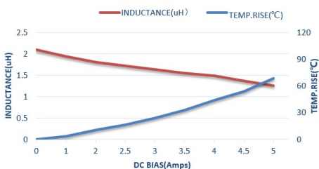
XRTC252010S2R2MBCA
