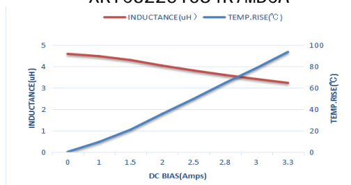
XRTC322510S4R7MBCA
