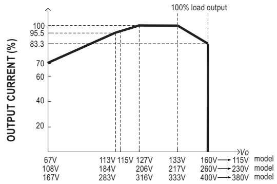
OUTPUT VOLTAGE
