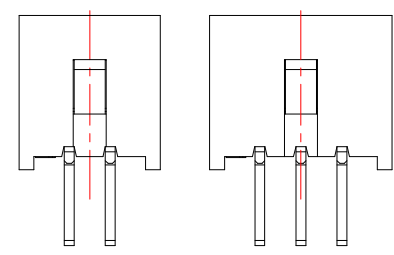
2 PIN 3 PIN LOCK CONFIGURATION (锁扣位置)
