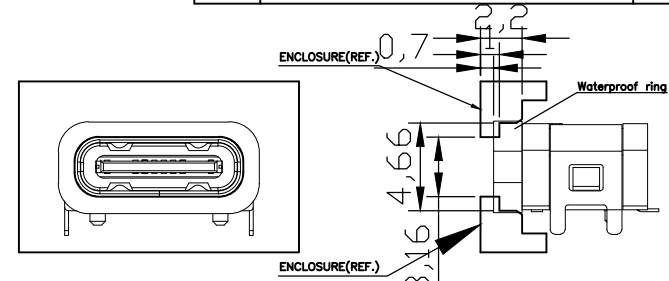
RECOMMENDED SCHEMATIC DRAWING OF CONNECTOR MATCH CHASSIS
