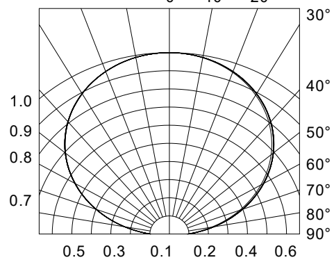
Fig.6-Radiation Diagram Ta=25°C
