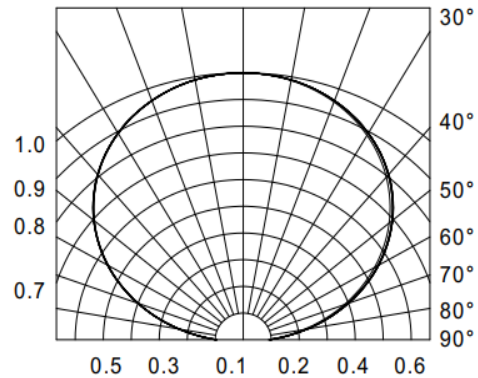
Fig.6-Radiation Diagram Ta=25°C
