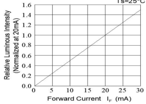
Fig.2-Relative Luminous Intensity vs. Forward Current Ts=25°C
