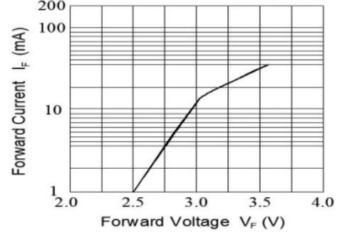
Fig.4-Forward Current vs. Forward Voltage Ta=25°C
