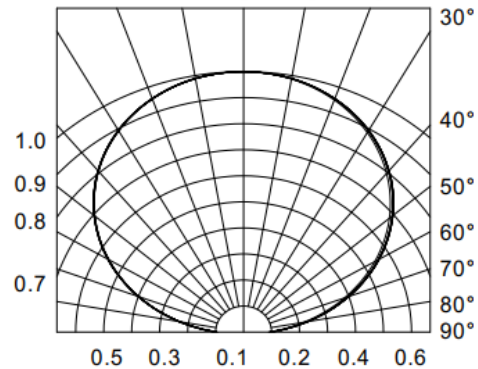
Fig.6-Radiation Diagram Ta=25°C
