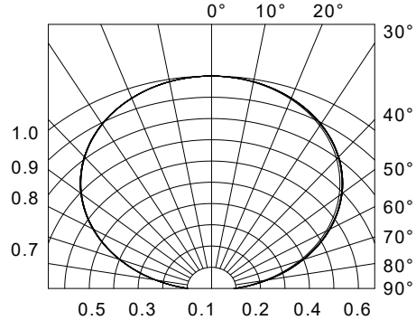
Fig.6-Radiation Diagram Ta=25°C
