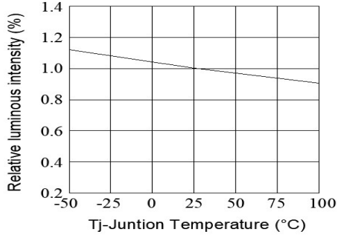
Fig.3-Relative Luminous Intensity vs. Junction Temperature
