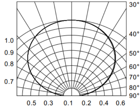
Fig.6-Radiation Diagram Ta=25°C
