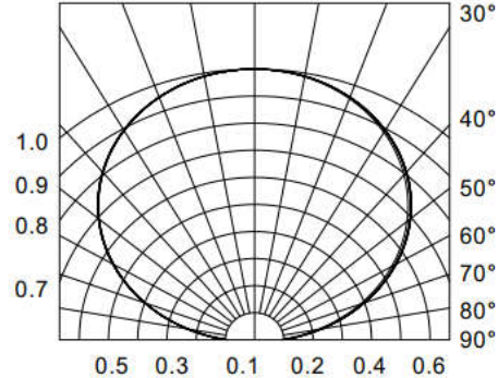
Fig.6-Radiation Diagram Ta=25°C
