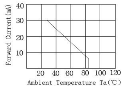
FIG. 6 Maximum Forward Current VS. Temperature
