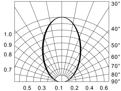
Fig.6-Radiation Diagram Ta=25°C
