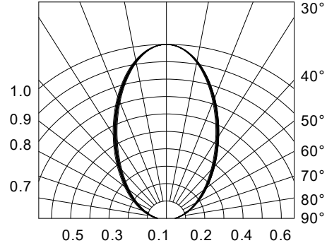
Fig.6-Radiation Diagram Ta=25°C
