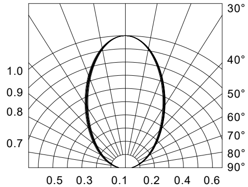
Fig.6-Radiation Diagram Ta=25°C
